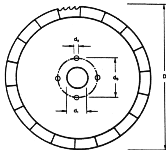
Segmental Saw Blade Specifications
